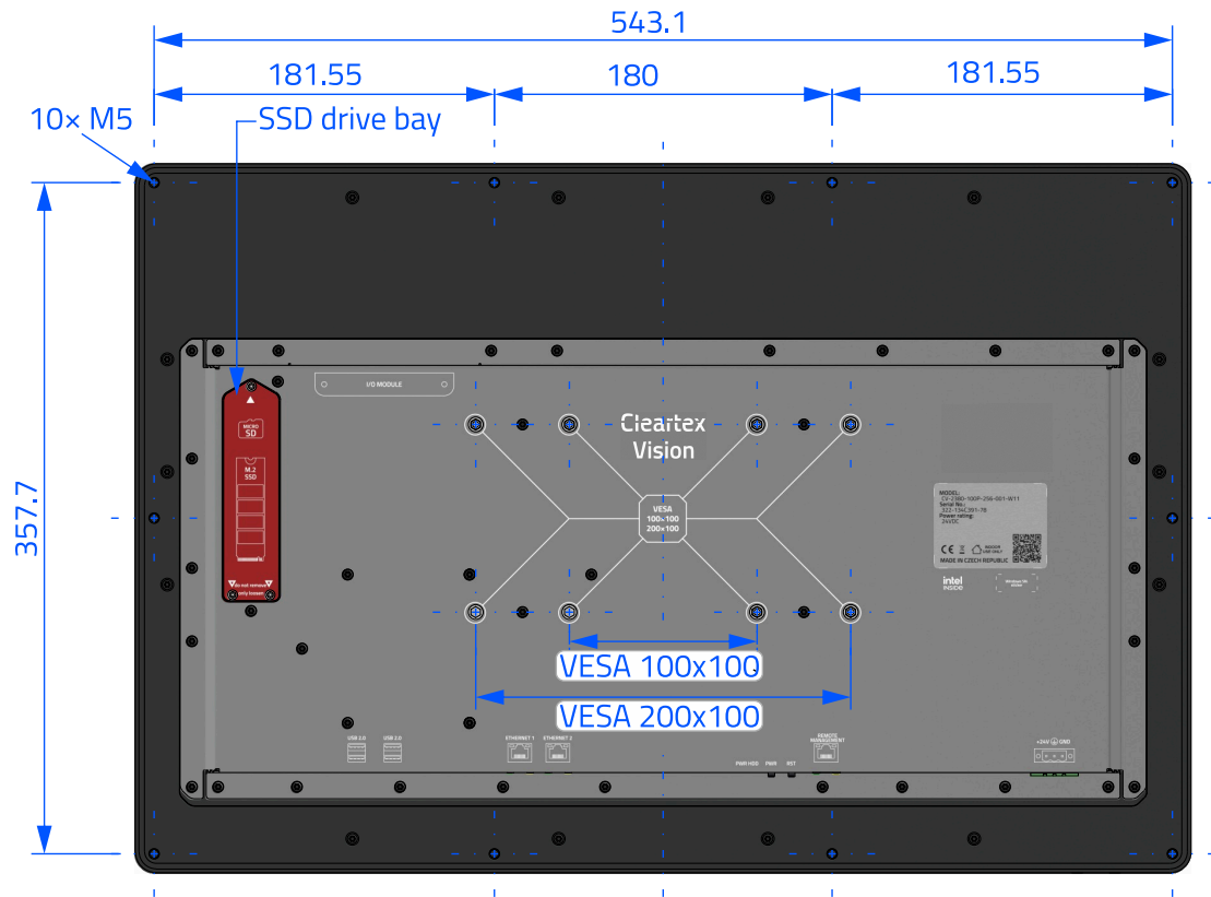
Image 14: Model 23.8" - back side drawing - passive cooling
