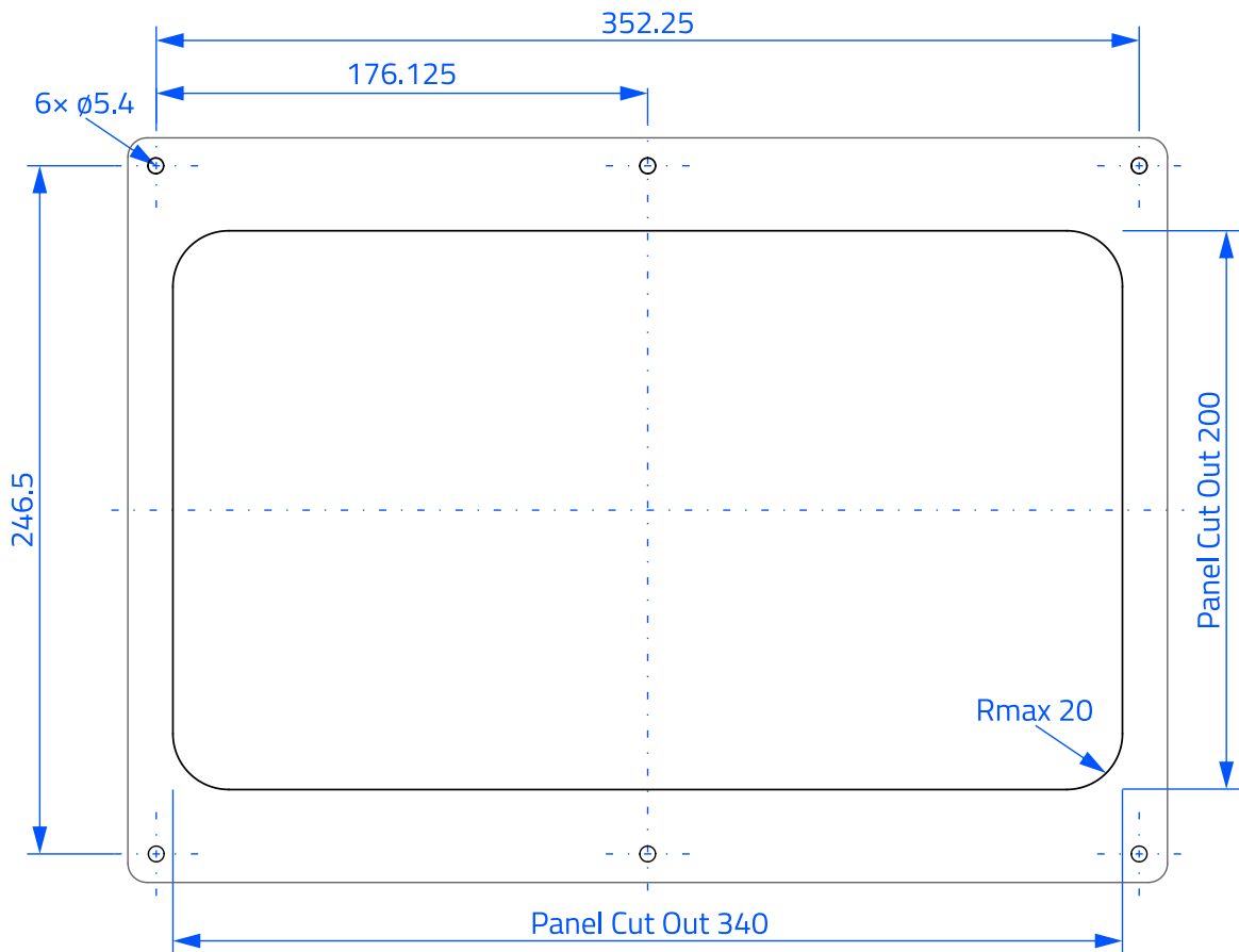
Image 25: Installation cutout drawing 15.6"
