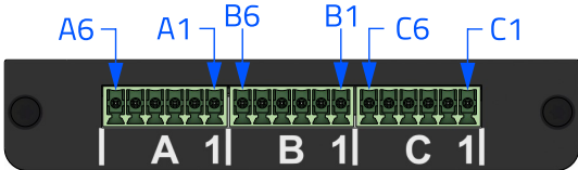
Image 22: IO-1 - inputs, outputs, relays, RS485
